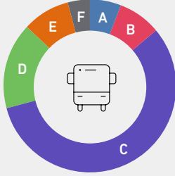
2021 GHG Emissions - by Source
