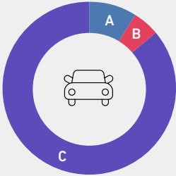
2021 GHG Emissions - by Scope
